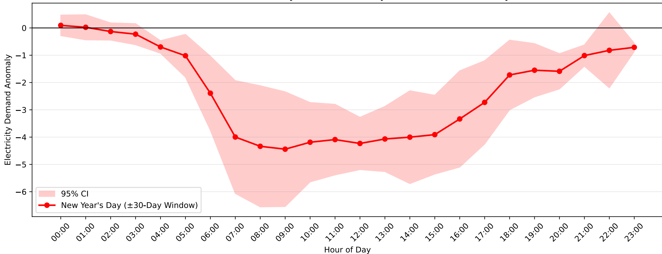
Beacon Hill Demand Anomaly: New Year's Day (2010–2011, \pm 30 -Day Window)
