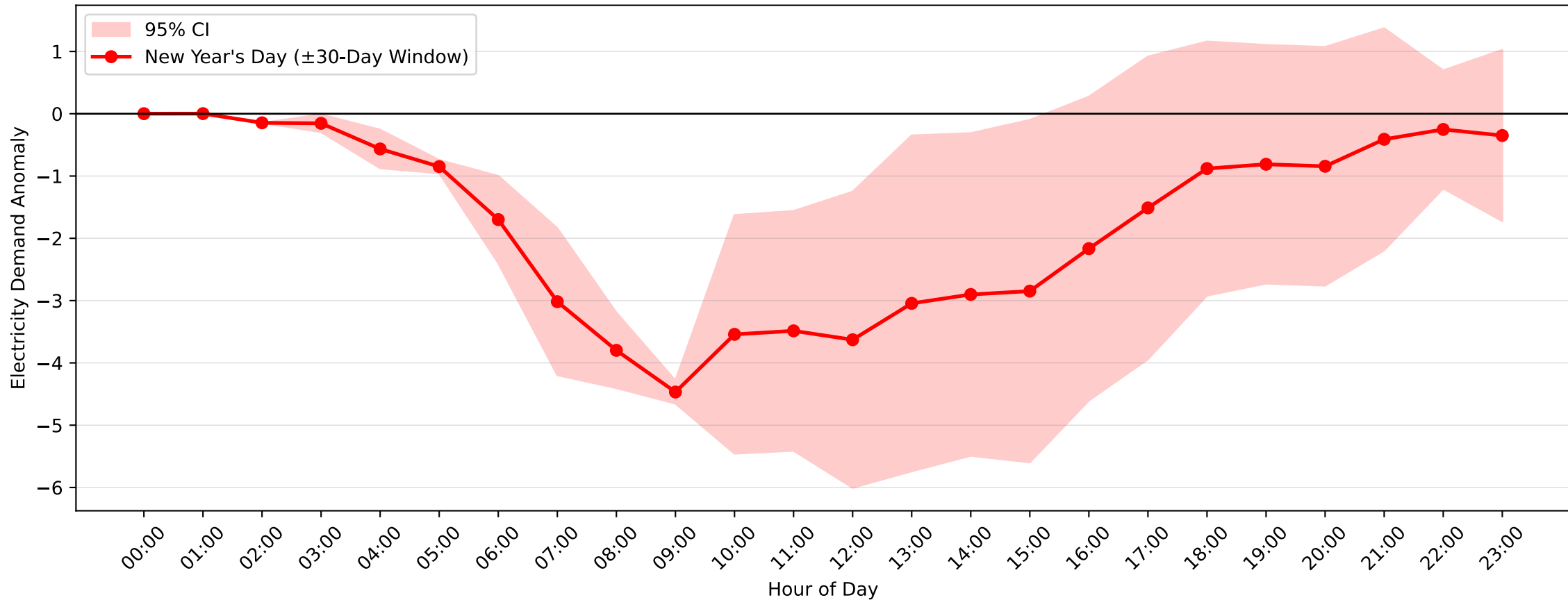
Beacon Hill Demand Anomaly: New Year's Day (2009–2010, \pm 30 -Day Window)
