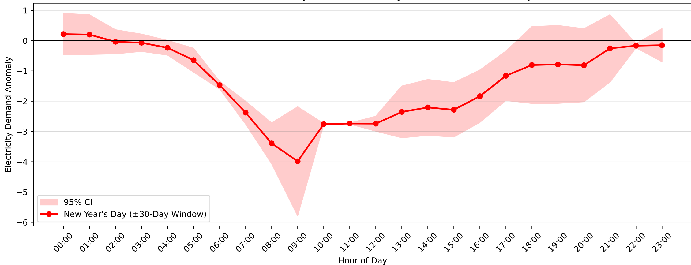
Beacon Hill Demand Anomaly: New Year's Day (2008-2009, \pm 30 -Day Window)
