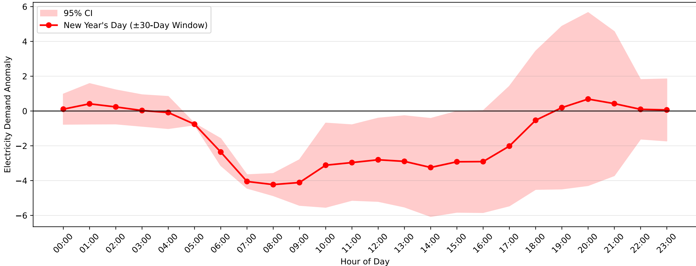
Beacon Hill Demand Anomaly: New Year's Day (2006–2007, \pm 30 -Day Window)
