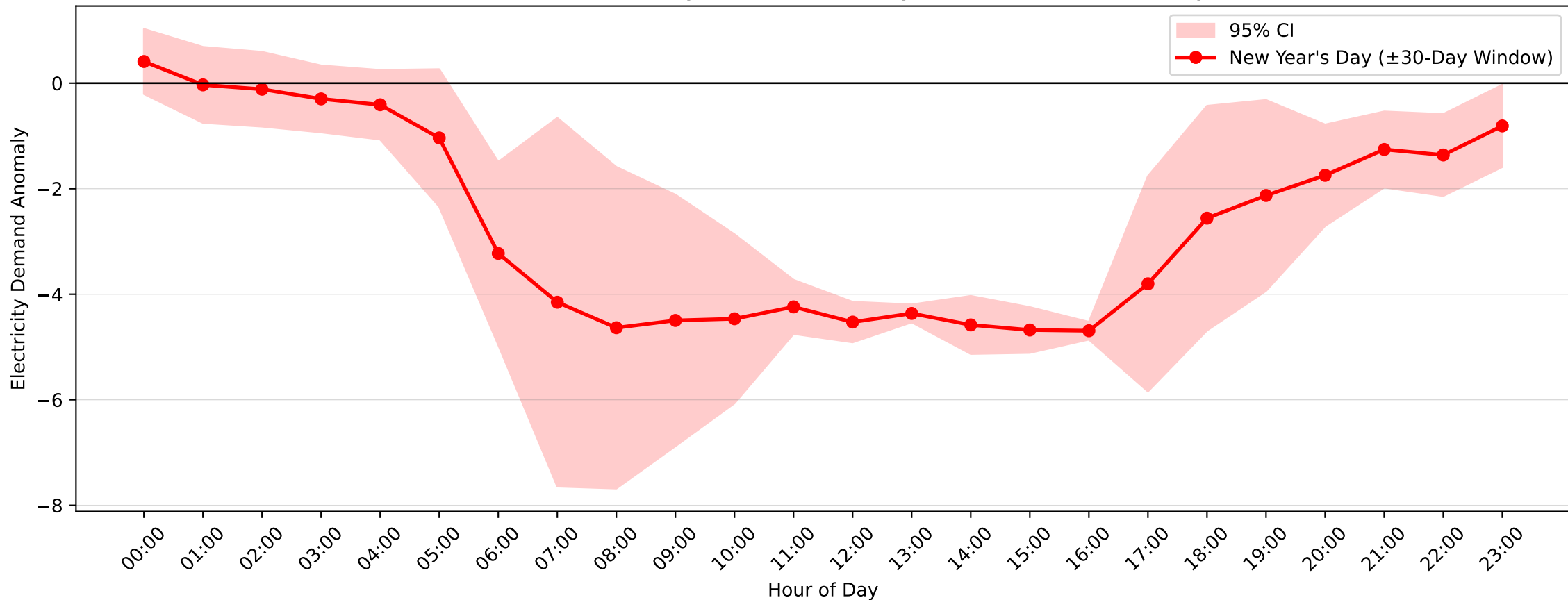
Beacon Hill Demand Anomaly: New Year's Day (2004-2005, \pm 30 -Day Window)
